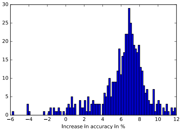
Figure: Comparison of a LSTM network with a feedforward neural network. Models are trained to predict the direction \{ -1, +1 \} of next mid-price move. Comparison for approximately 500 stocks and out-of-sample results reported for June-August, 2015.
